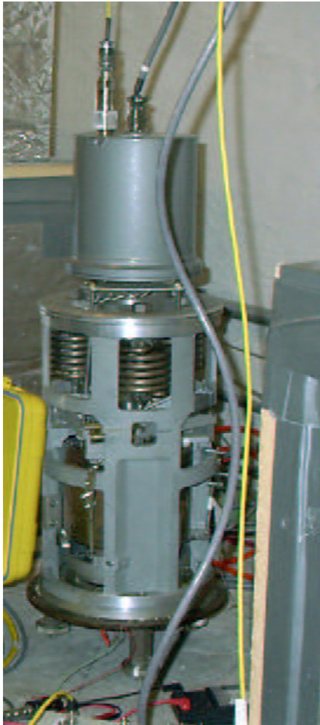
Figure 11.6: Simple vertical shake table, constructed using a Johnson-Matheson Model 6840 short-period seismometer, with a PMD sensor mounted on top of the shake table for testing.
