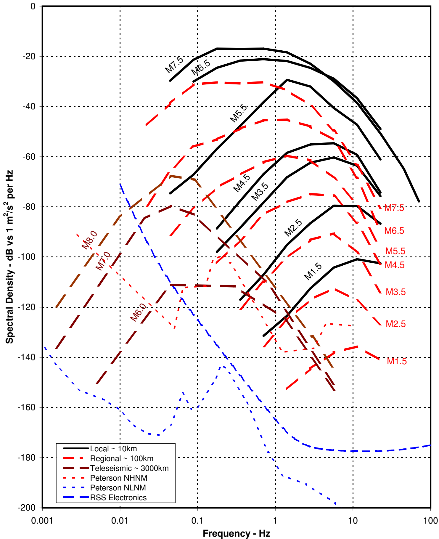
Velocity power density vs Frequency Derived From Clinton and Heaton, Seis.Res.Let. 2002,v73,n3 and Peterson, USGS Open File Report 93-322, 1993
