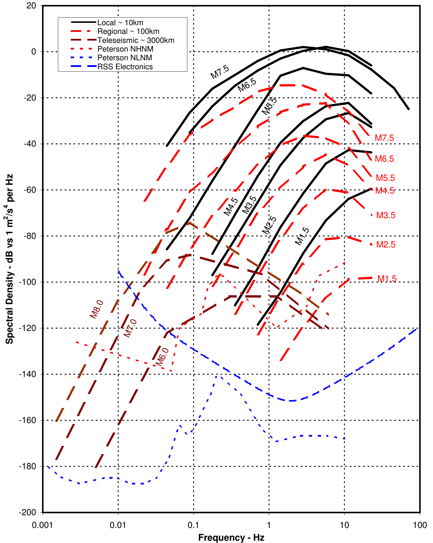
Acceleration power density vs Frequency Derived from Clinton and Heaton, Seis.Res.Let. 2002,v73,n3 and Peterson, USGS Open File Report 93-322, 1993
