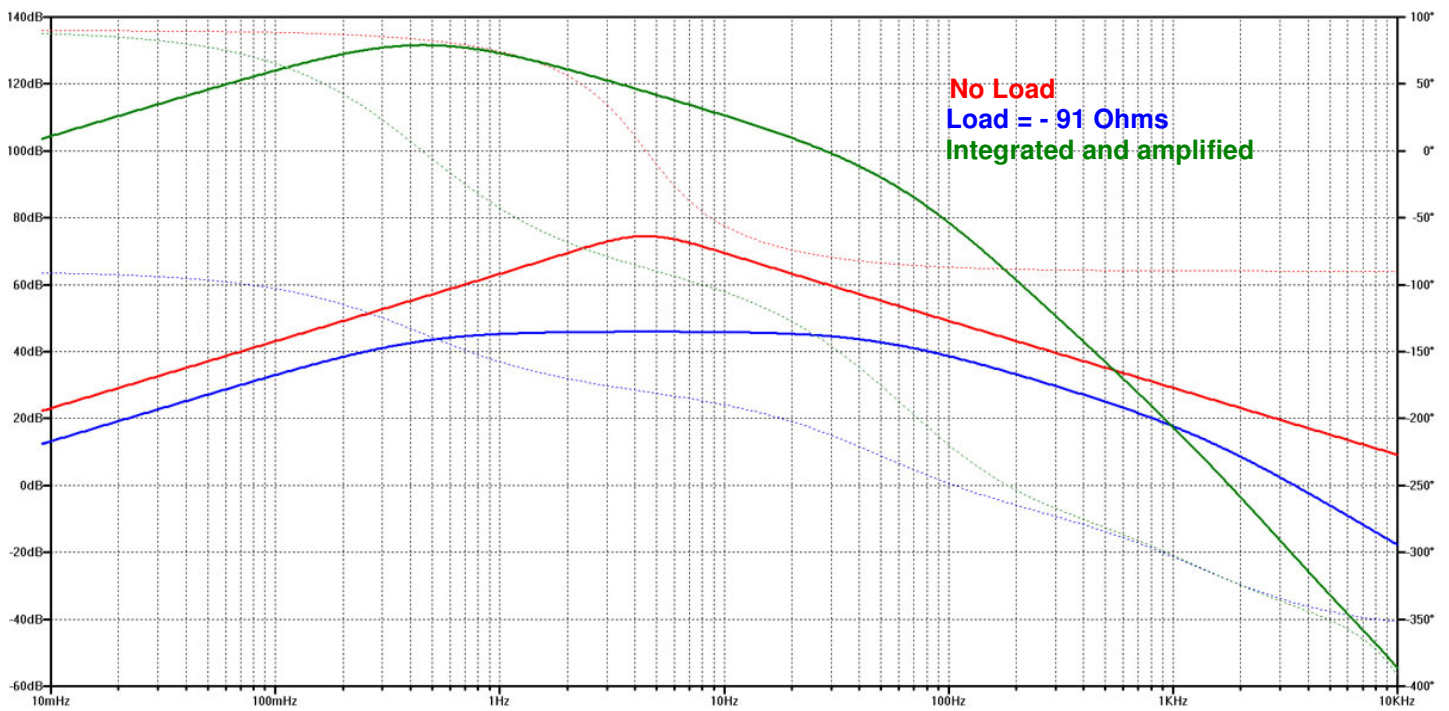
PS-4.5B Geophone acceleration response - dB vs 1 V / m/s 2
