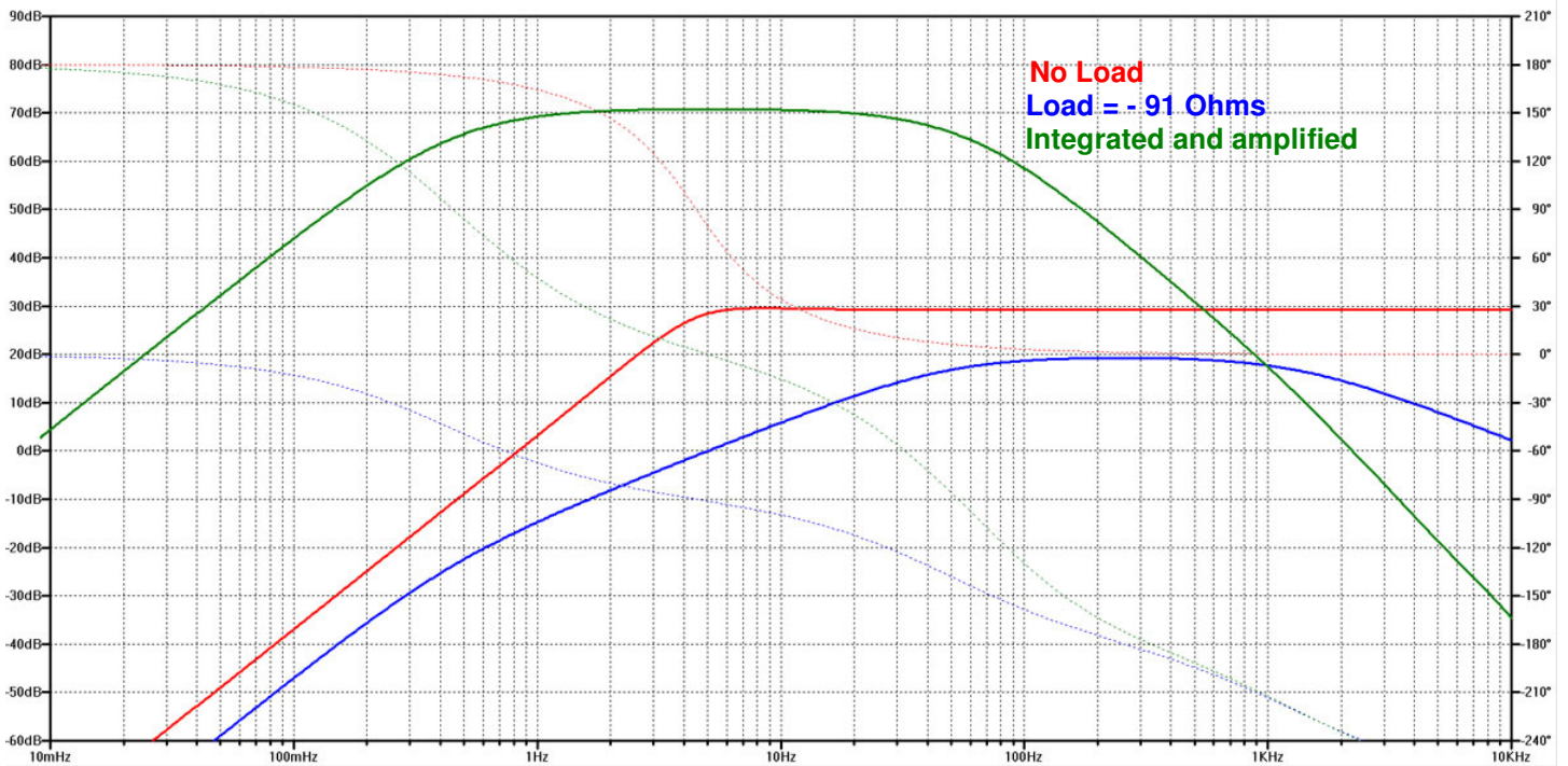
PS-4.5B Geophone velocity response - dB vs 1 V / m/s
